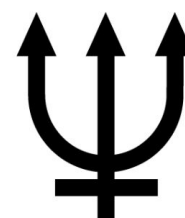
Neptune
